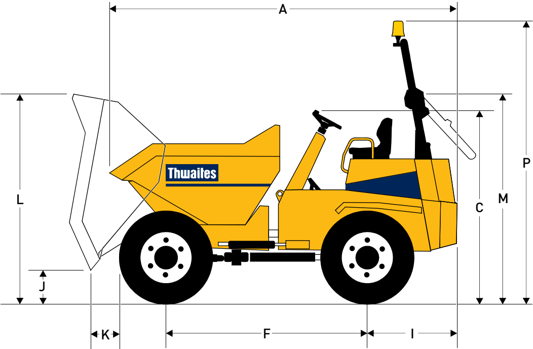
Dimensions (mm)
